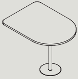
CTP-2190-4 W 1000 D 730 H 700 (FOR 4P ARC OR STRAIGHT W/ ARMS)
