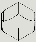
PC1 W 730 D 730 H 760 S 440 W 28.7" D 28.7" H 30.0" S 17.3"
