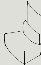
PHB30-R W 1090 D 920 H 1350 S 440 IN Ø2920 / OUT Ø4380 W 42.9" D 36.2" H 53.1" S 17.3" IN Ø115.0" / OUT Ø172.4"
